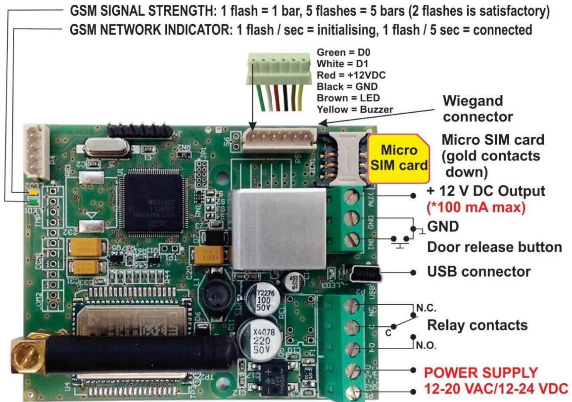
Figure 1: WLOCK: Connection diagram
