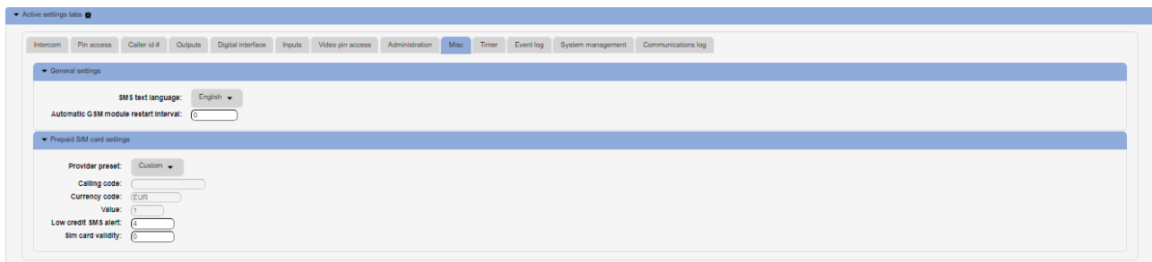
Figure 17: WEB Server-Misc
